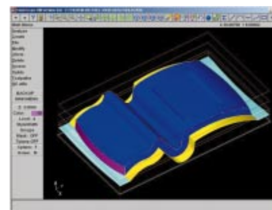
The seamless fit of all four layers of the ATM mold are graphically evident in this solid model.
